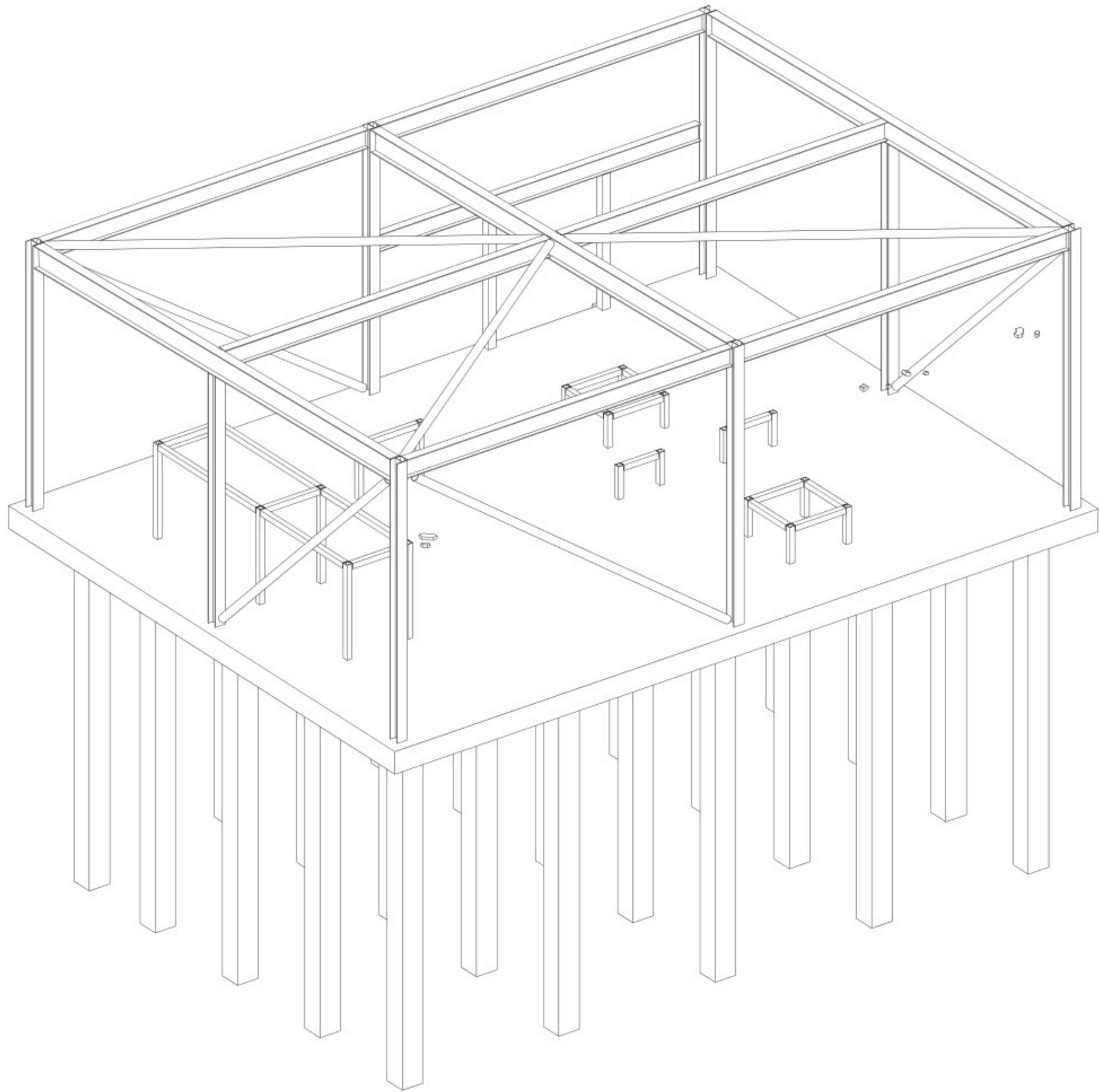
1 3D VIEW WMB AND FPA - 3D-AANZICHT WMB EN FPA
