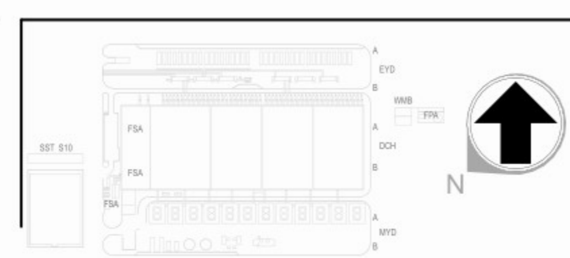
FOUNDATION LAYOUT (INDELING FUNDERING) Scale / Schaal 1 : 100
