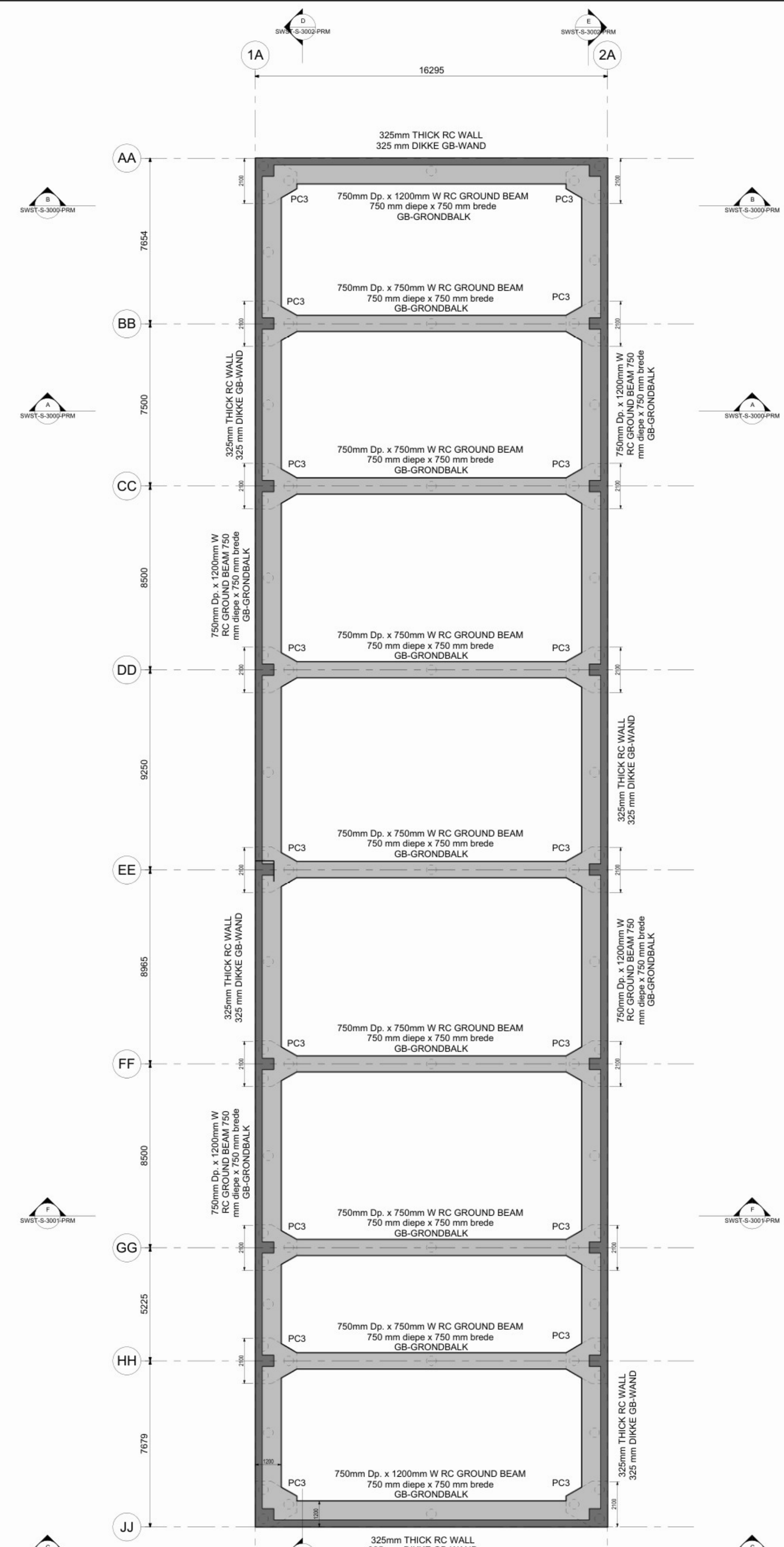
FOUNDATION LAYOUT (INDELING FUNDERING) Scale / Schaal 1 : 100
