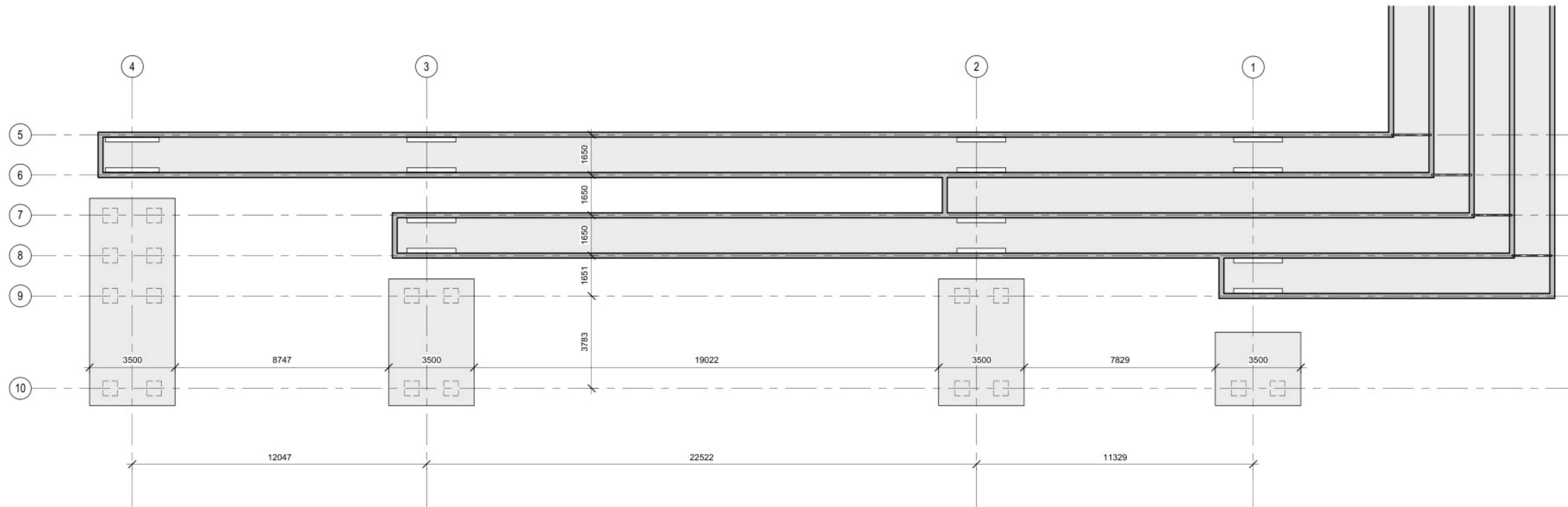
1 TRESTLE FOUNDATION LAYOUT - TRESTLE INDELING FUNDERING 1 : 100
