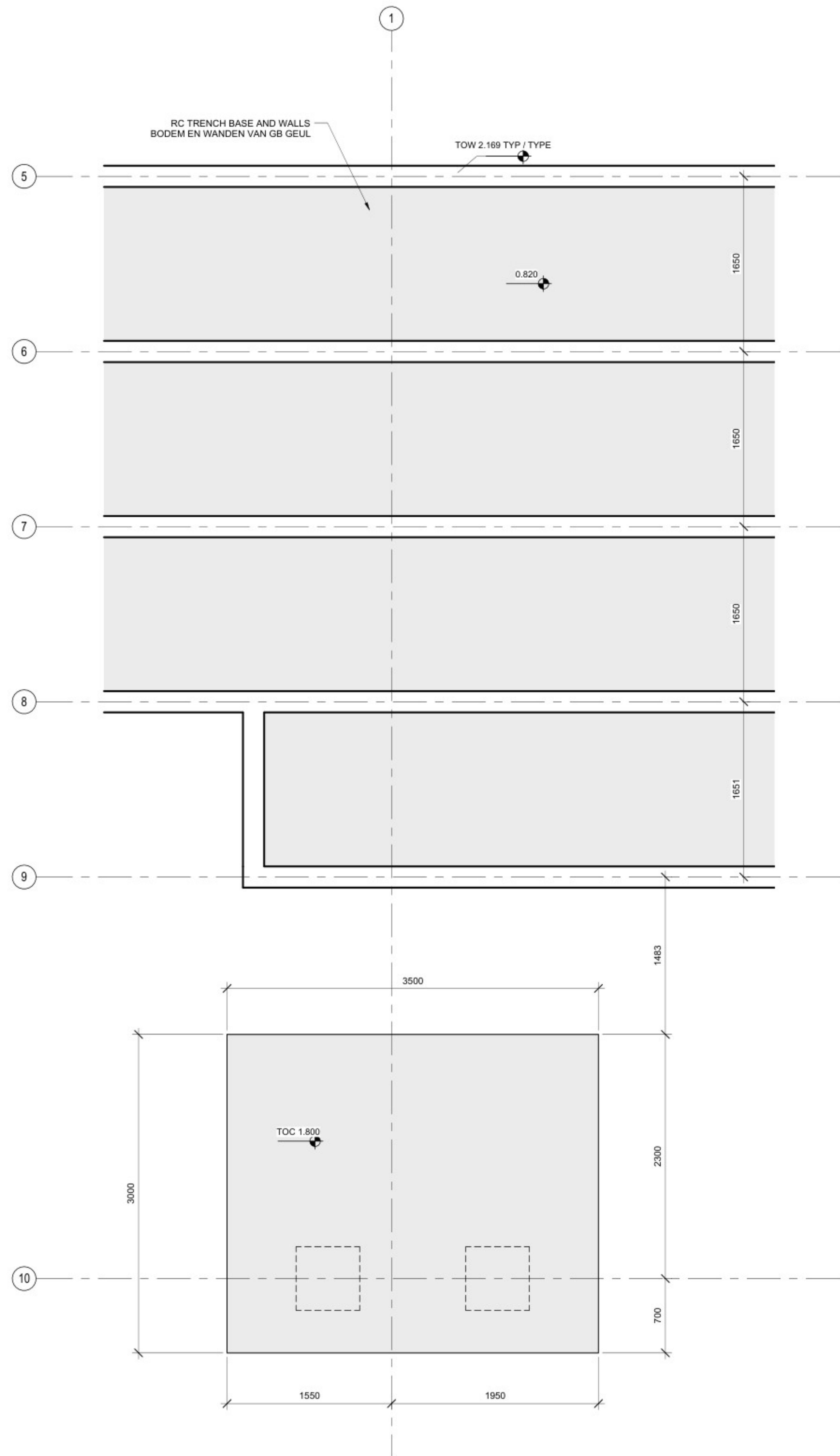
2 TRESTLE TYPICAL FOUNDATION SETTING OUT - TRESTLE TYPISCHE UITZETTING VAN FUNDERING 1 : 25
