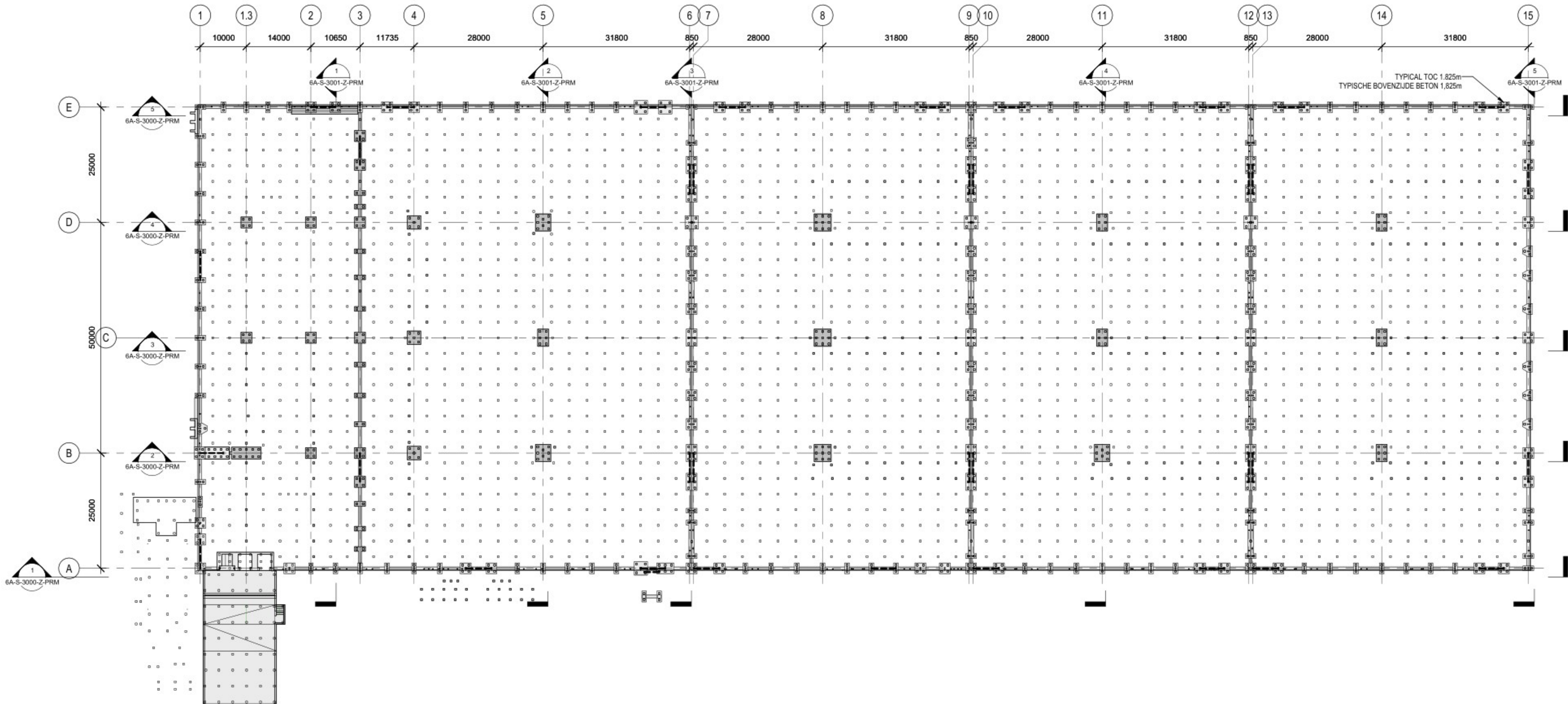
DC PILE CAP PLAN (PAALMUTSENPLAN DC) 1:500
