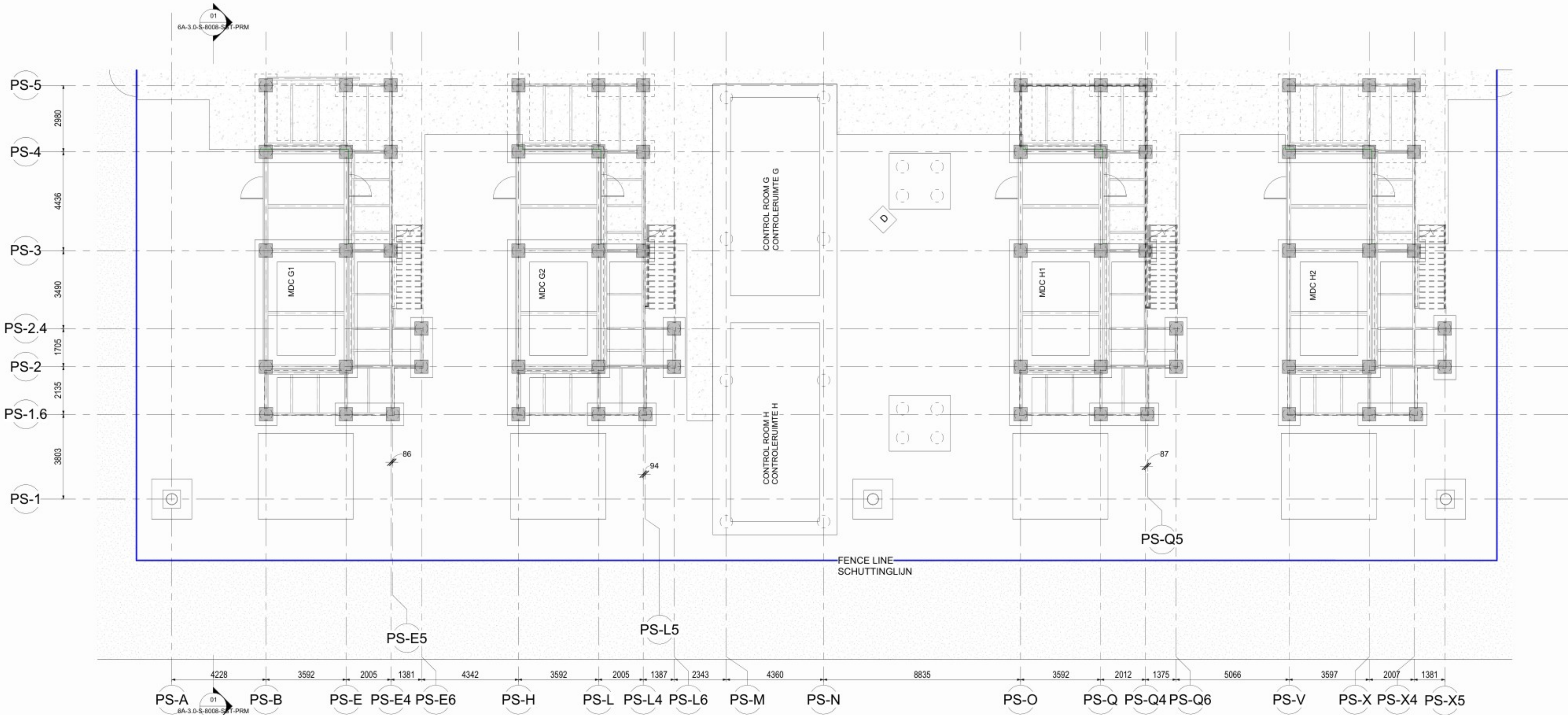
INTERFACE BETWEEN EMEA PERUN AND EXTERNAL SITE TRESTLE - INTERFACE TUSSEN EMEA PERUN EN EXTERN TERREINSCHRAAG SCALE/SCHAAL 1: 100
