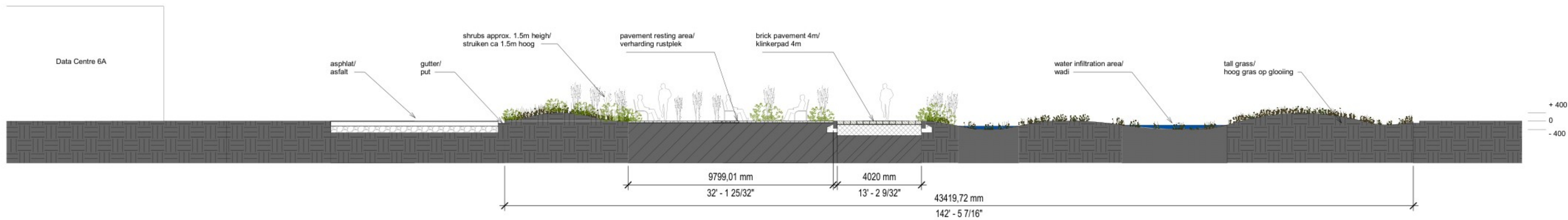
1 SECTION C - RESTING PLACE VISTA/ DOORSNEDE C - RUSTPLEK AS 1 : 100
