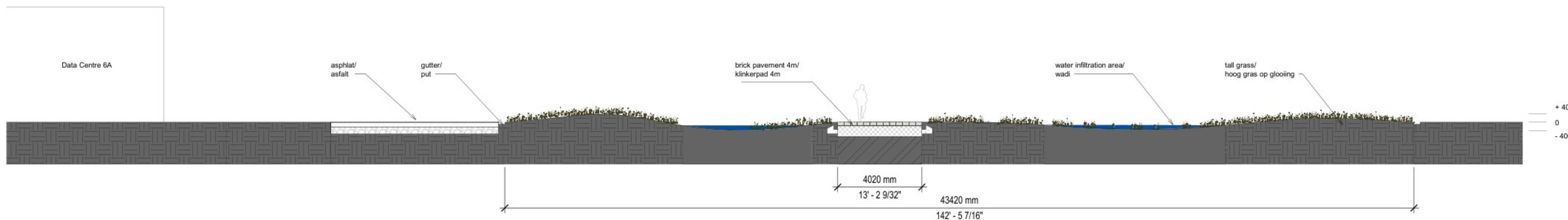
2 SECTION B - VISTA/ DOORSNEDE B - AS 1 : 100
