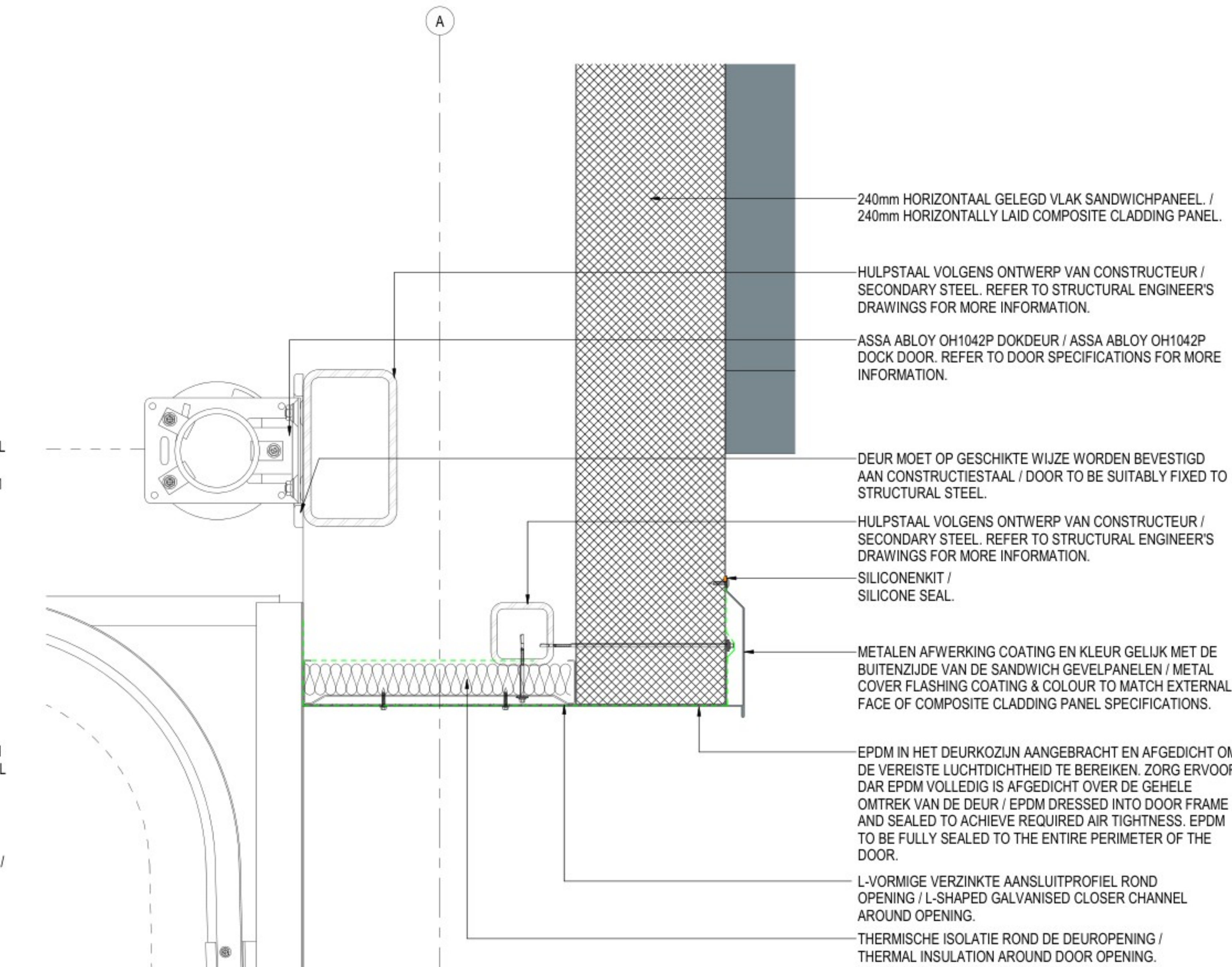
PRINCIPEDETAIL OVERHEADDEUR / SECTIONAL DOOR TYPICAL DETAIL
