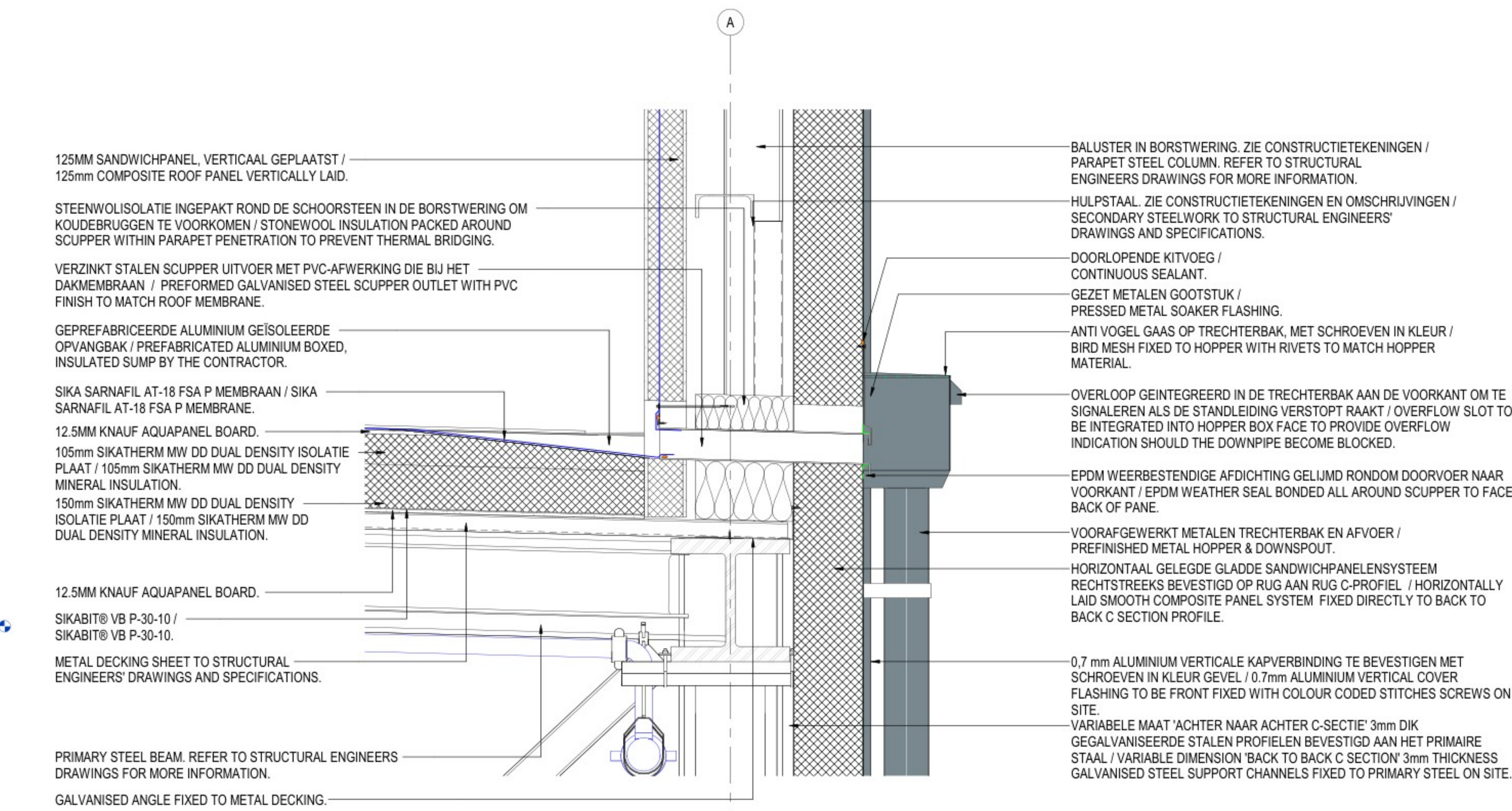
DETAIL DAKOPSTAND - HEMELWATERAFVOER / RAIN WATER PIPE PARAPET DETAIL
