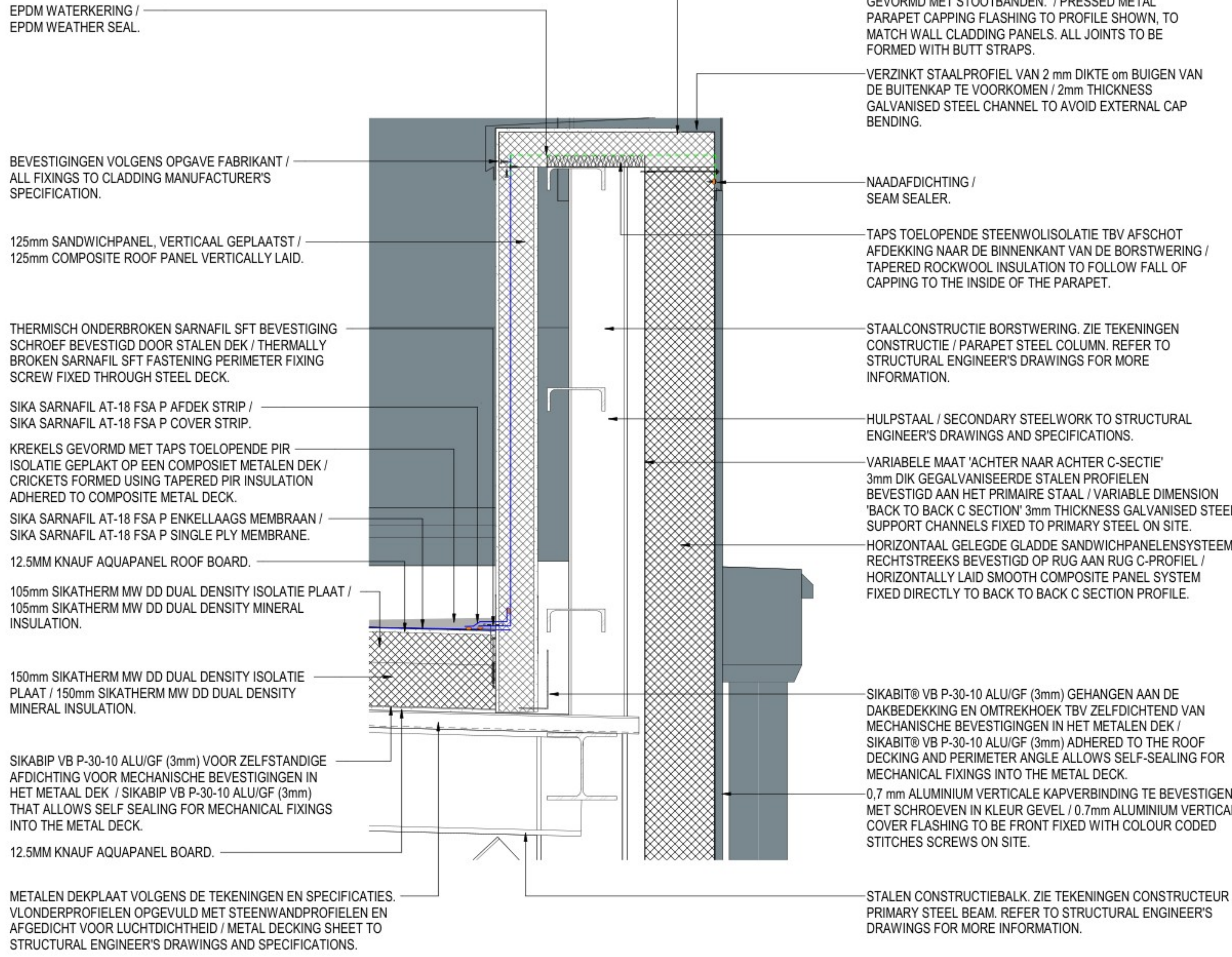
PRINCIPEDETAIL DAKOPSTAND / PARAPET TYPICAL DETAIL
