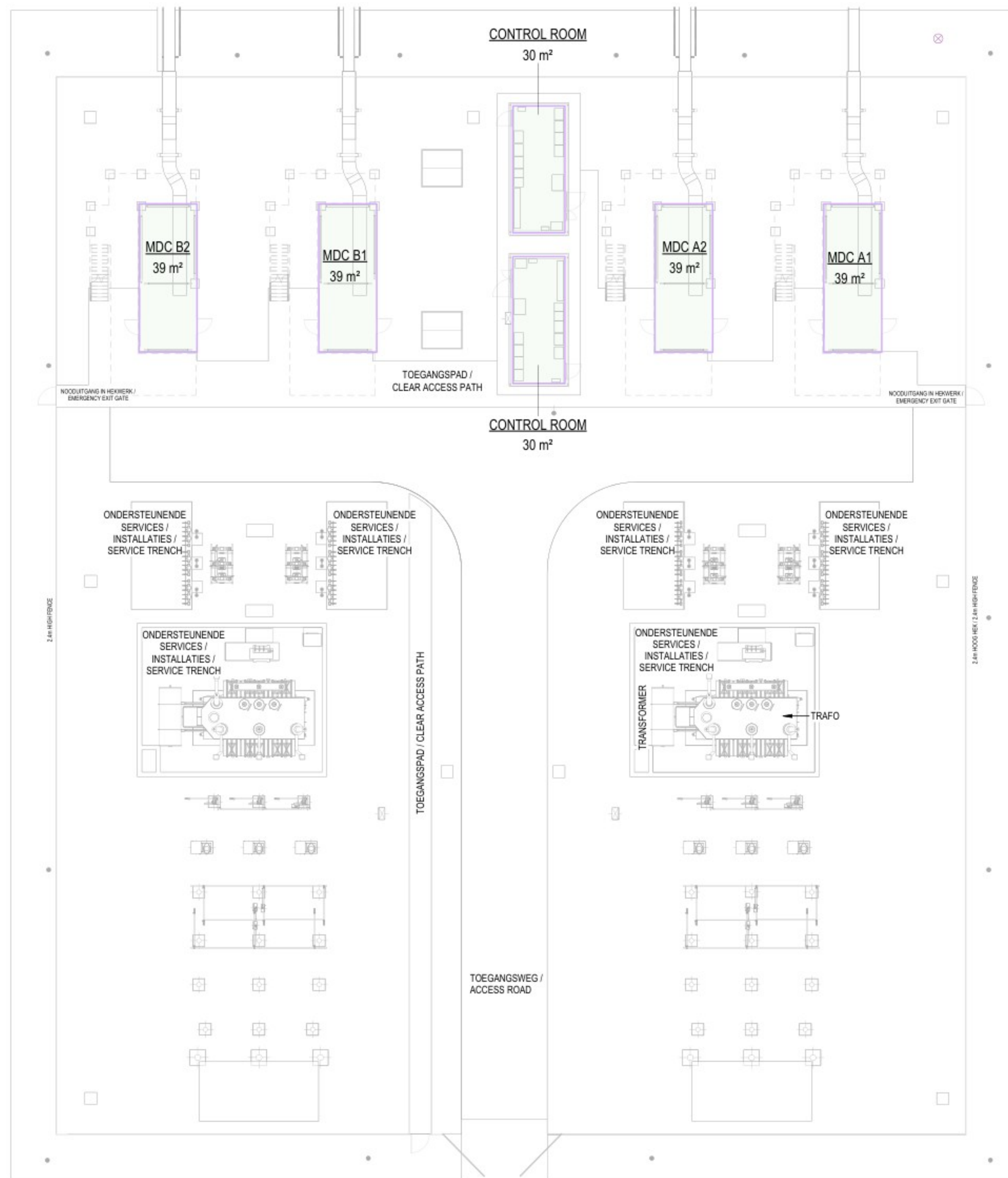
1 BEGANE GROND / GROUND FLOOR 1 : 200
