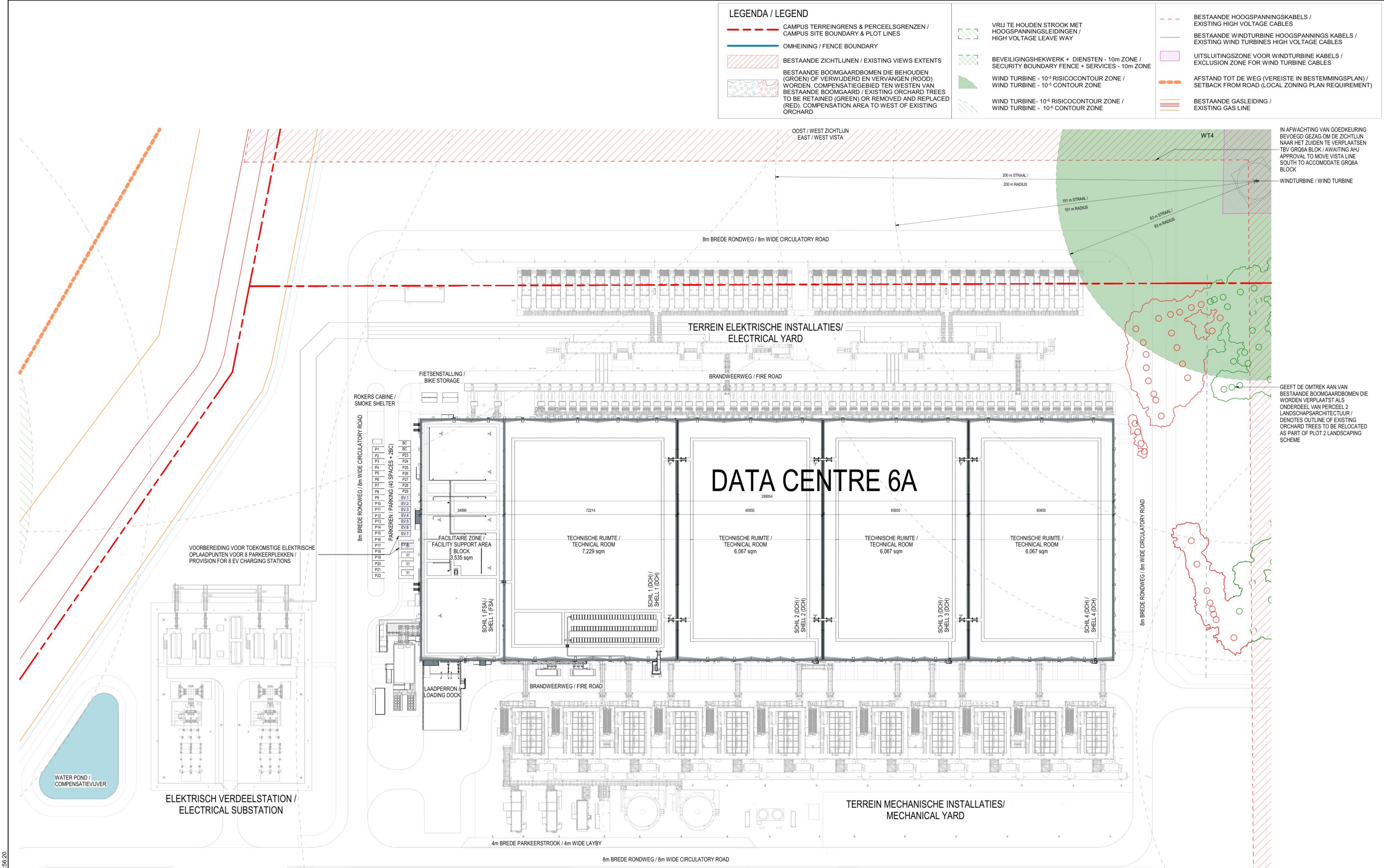
1 BOUWKUNDIGE SITUATIE - NIEUW / ARCHITECTURAL SITE PLAN BUILDING PROPOSED SITUATION 1 : 500
