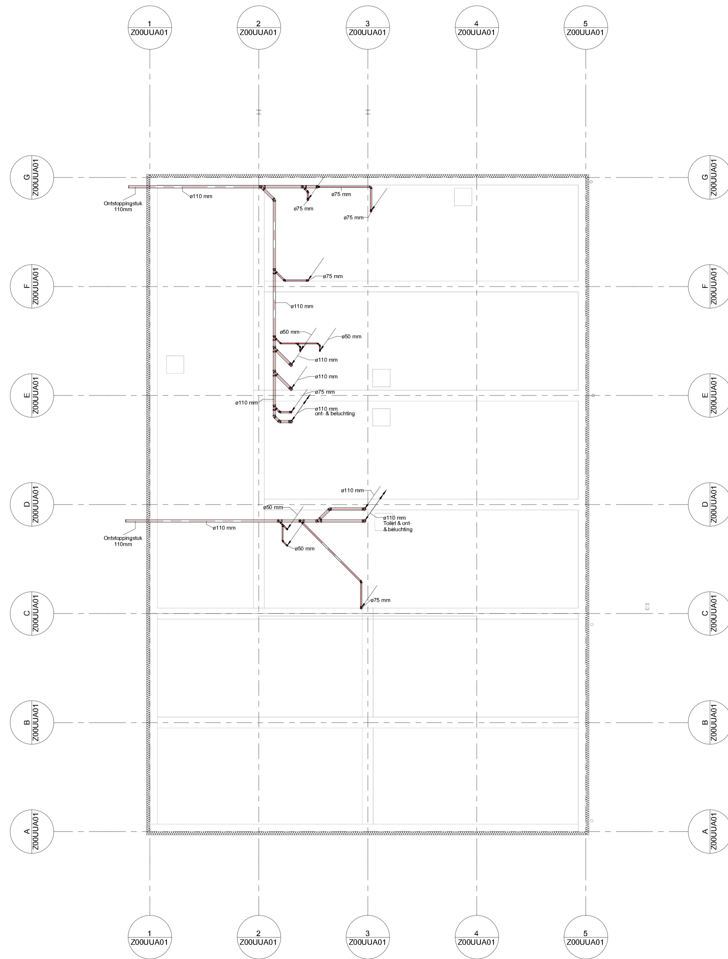
1 RIOLERING FUNDERING 1 : 100
