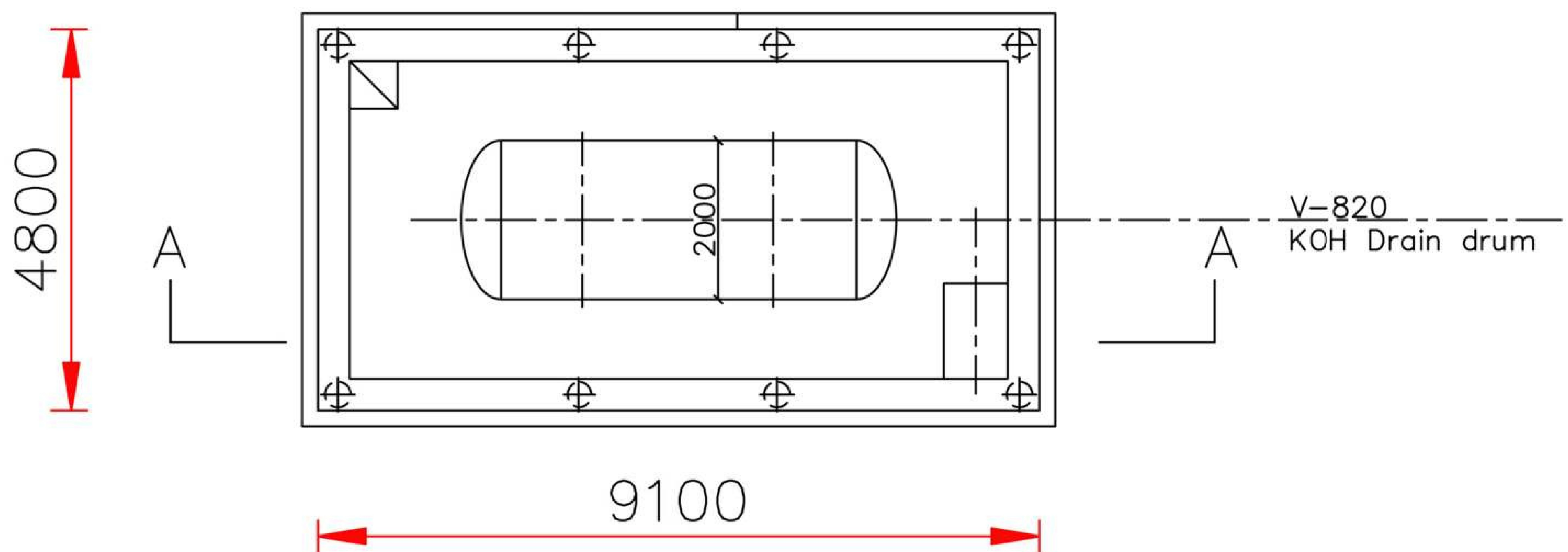
FOUNDATION PLAN
