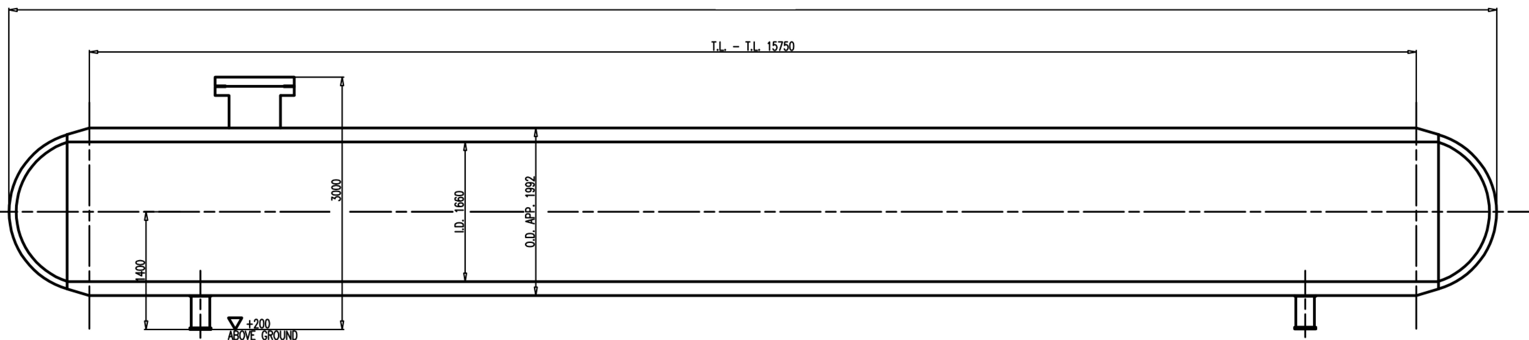
HYDROGEN STORAGE BULLETS – T-512 A/B/C
