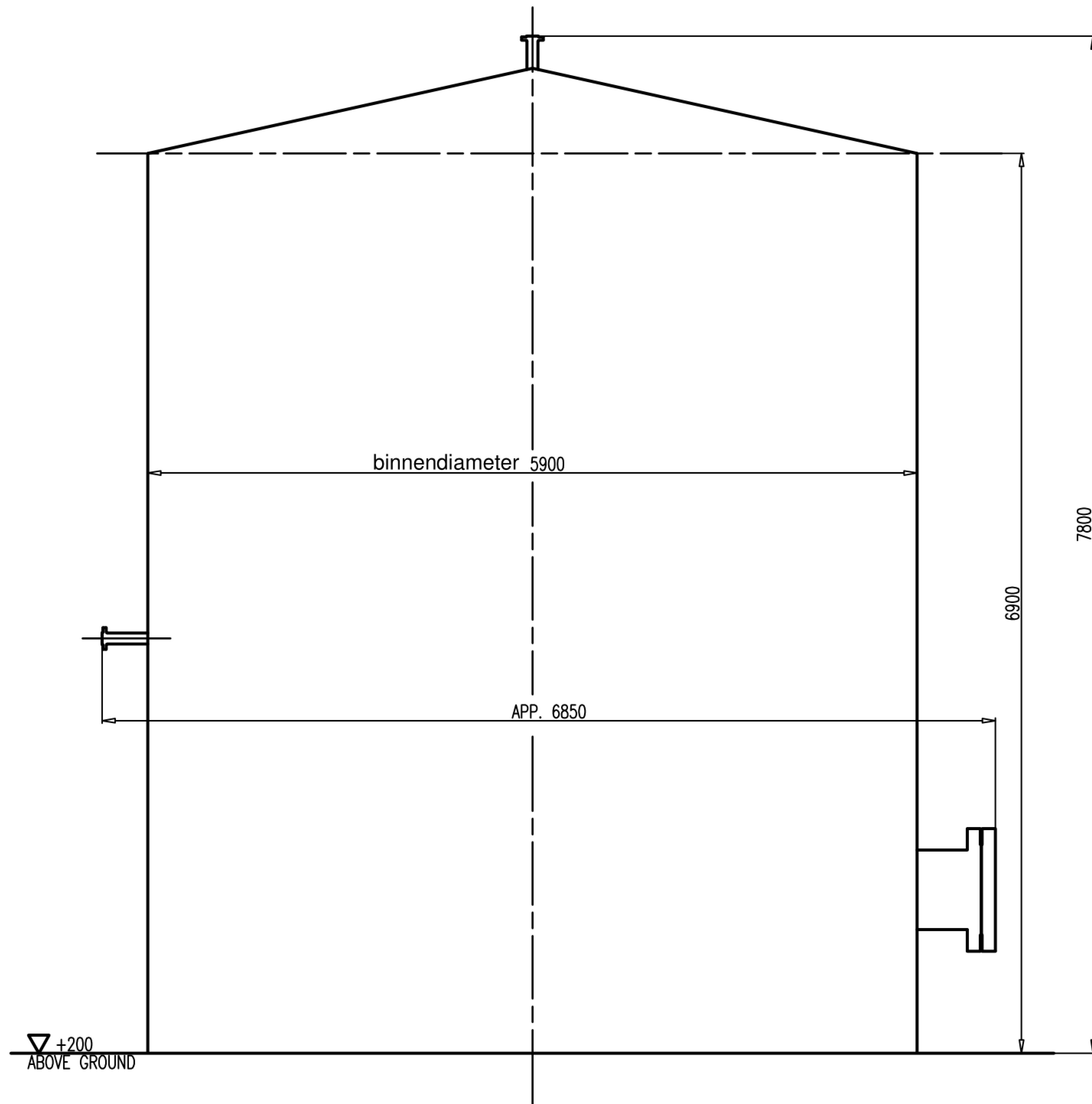
ULTRA PURE WATER TANK – T-841
