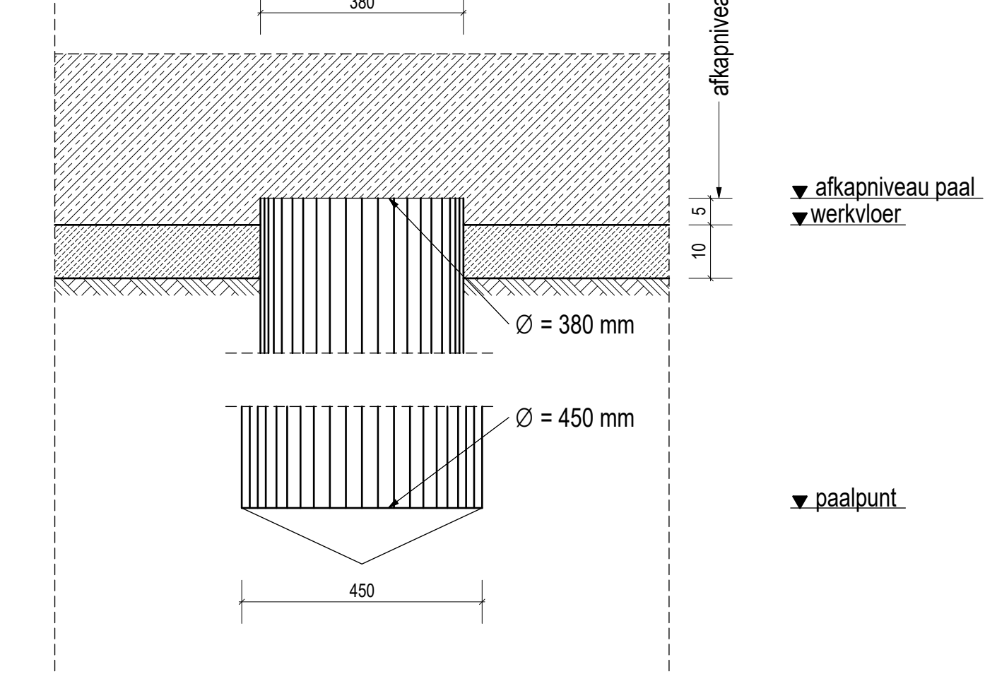
Detail Paal M 1:10
