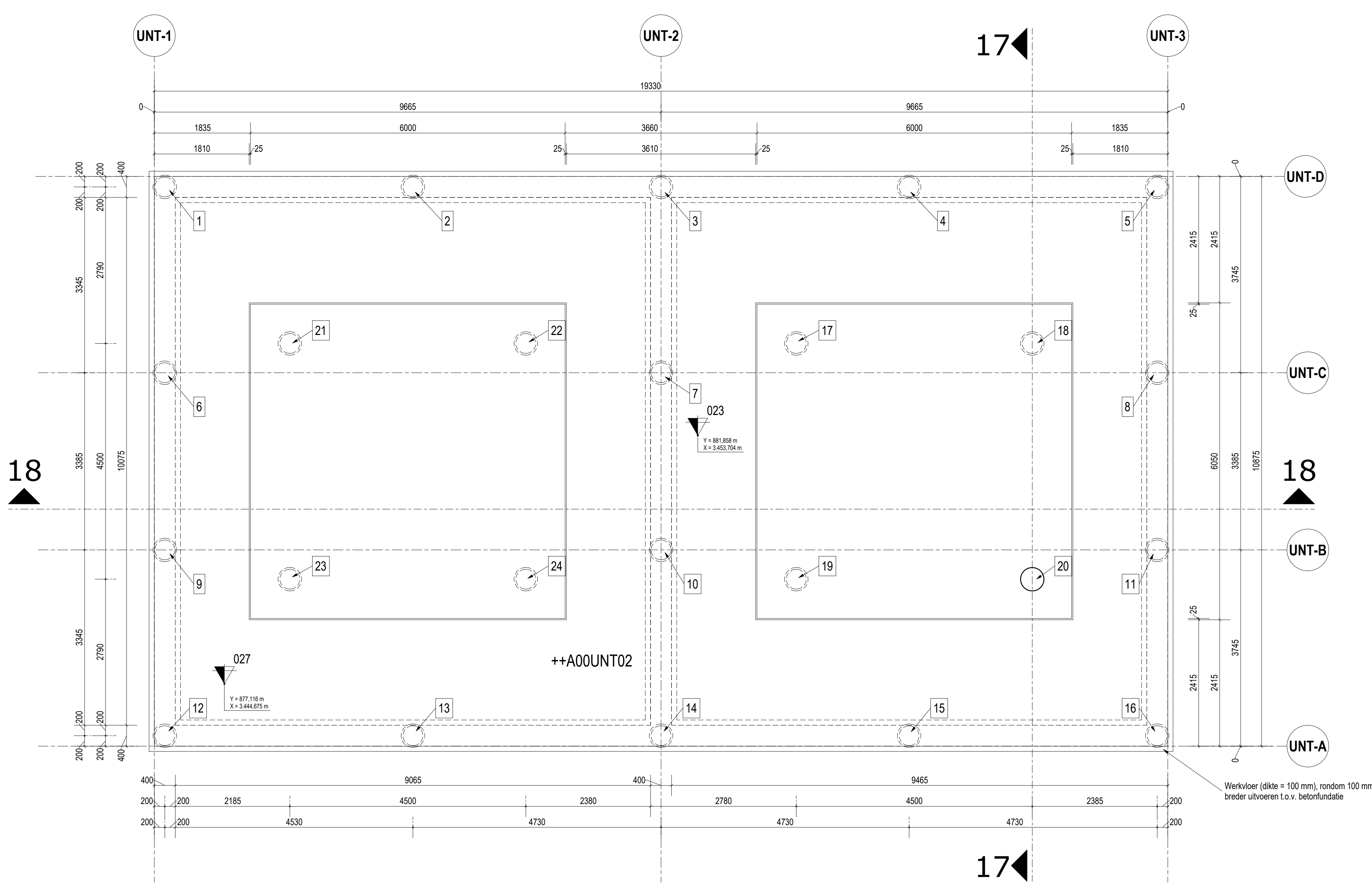
Fundatie Compressor Building M 1:50
