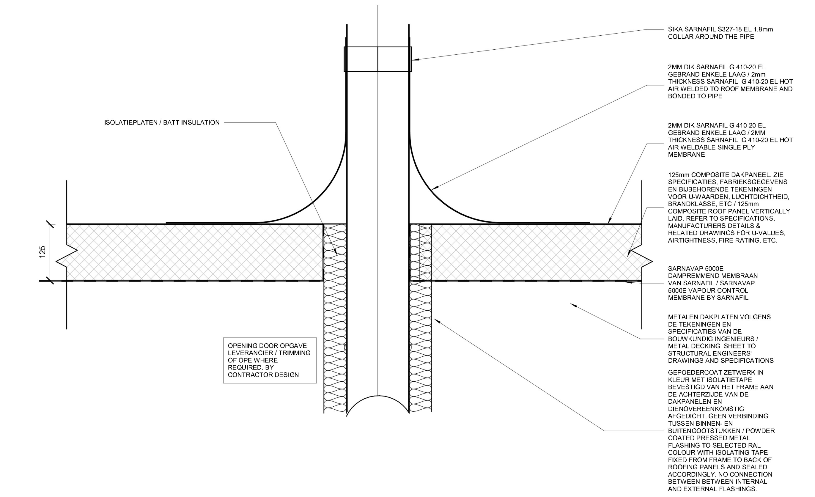
2 PRINCIPEDETAIL DAK DOORGANG / EXTERNAL ROOF - PIPE PENETRATION 1 : 5
