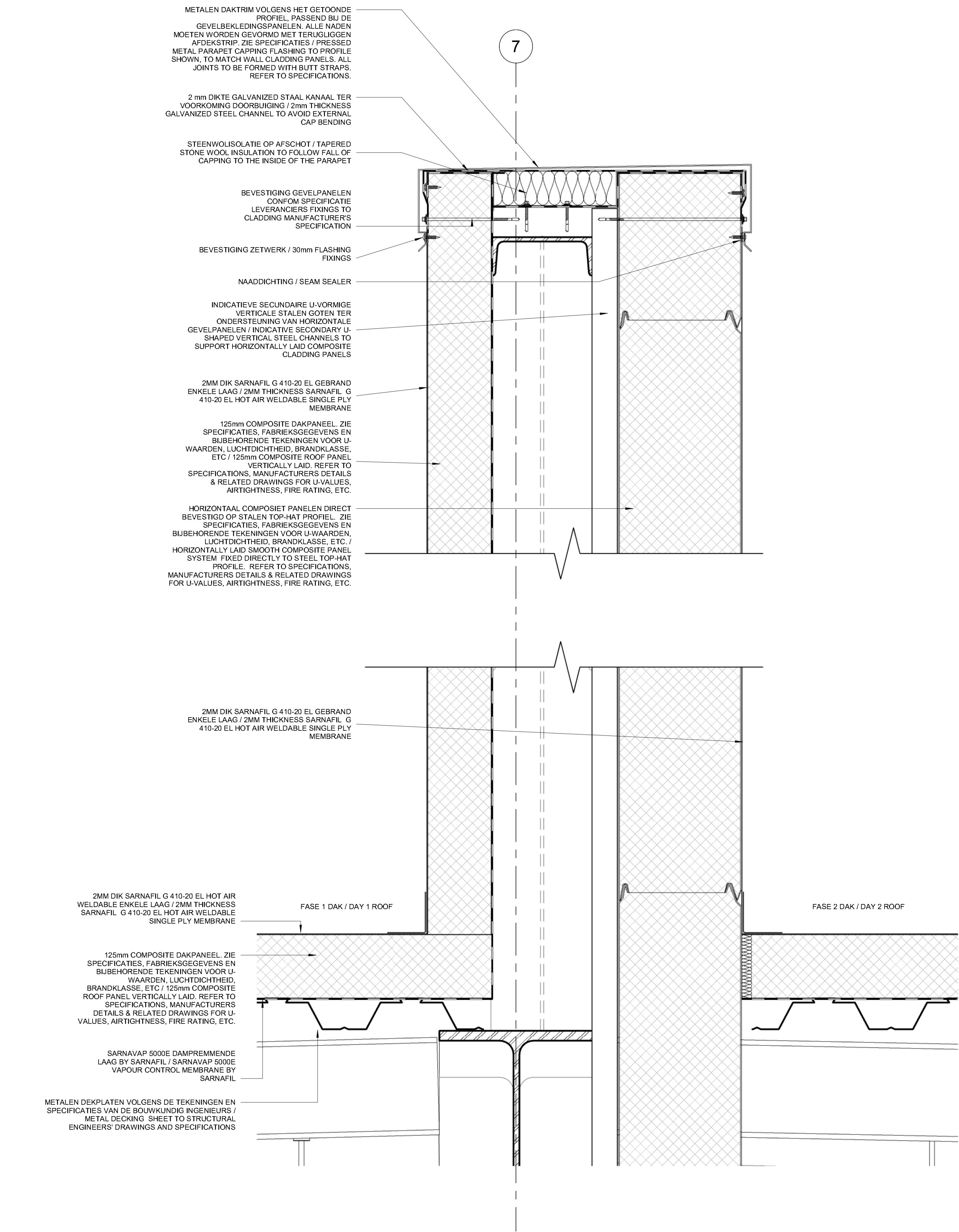
1 DAKOPSTAND FASE 1-2 / PARAPET DAY 1-2 1 : 5
