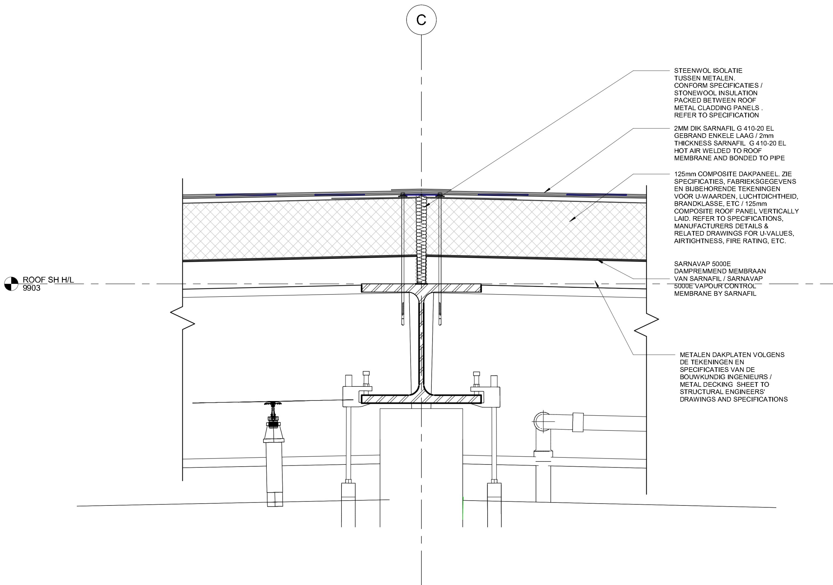
3 PRINCIPEDETAIL DAK / EXTERNAL ROOF - TYPICAL ROOF RIDGE DETAIL 1 : 5
