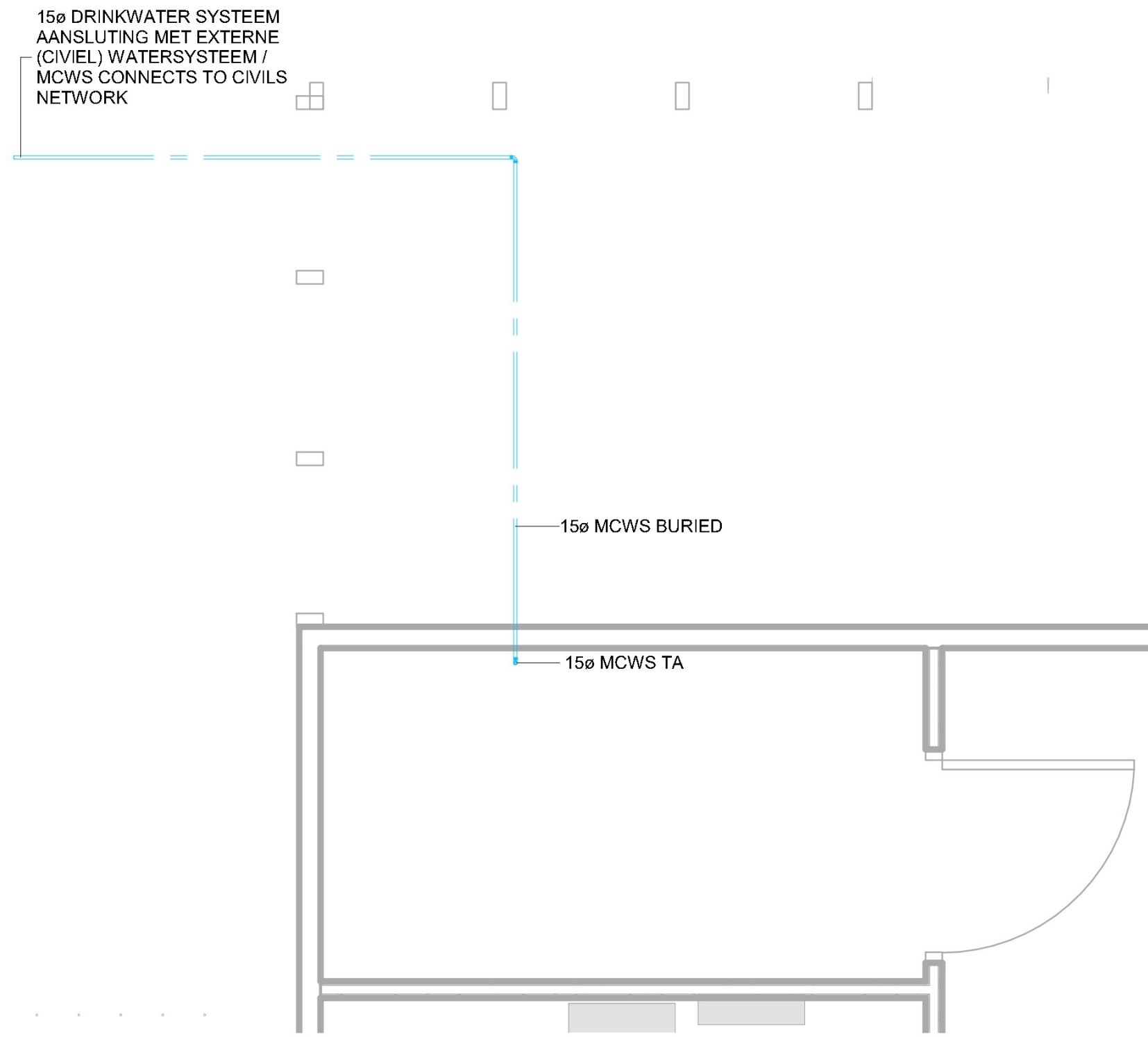
④ PLUMBING BELOW GROUND PLAN - WATER SERVICES / NANO ENTRANCE LEIDINGWERK SITUATIETEKENING 1 : 25
