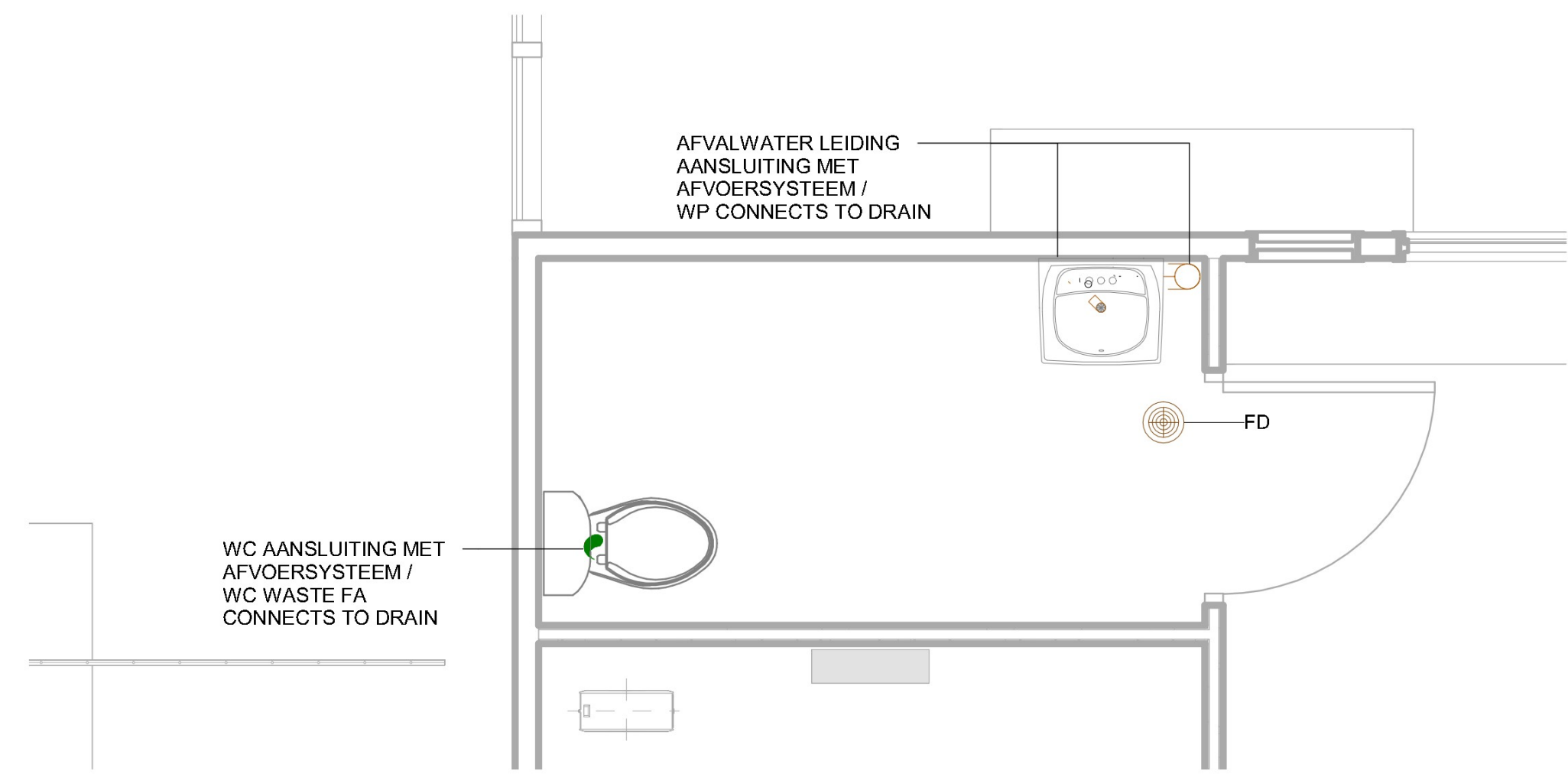
③ PLUMBING ABOVE GROUND PLAN - DRAINAGE / PLATTEGROND WATERAFVOER (BOVENGRONDS) 1 : 25
