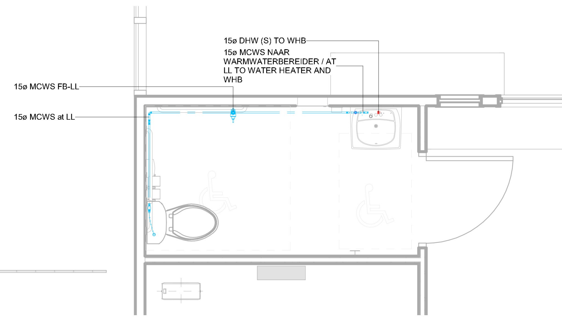
⑤ PLUMBING ABOVE GROUND PLAN - WATER SERVICES / PLATTEGROND WATERAANSLUITING (BOVENGRONDS) 1 : 25
